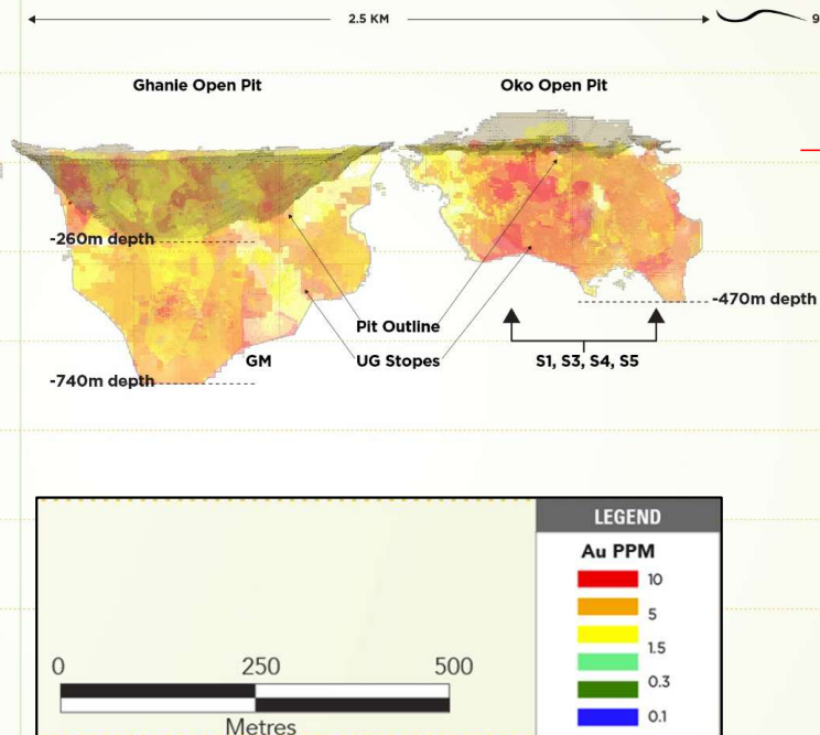
Oko Project Long Section Looking West: Oko & Ghanie Deposits OP& UG Mining Constraints with Blocks
