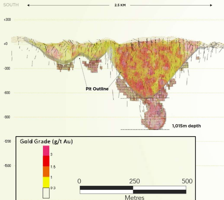
Figure 16.28: Mine Development Longitudinal View - Looking West
